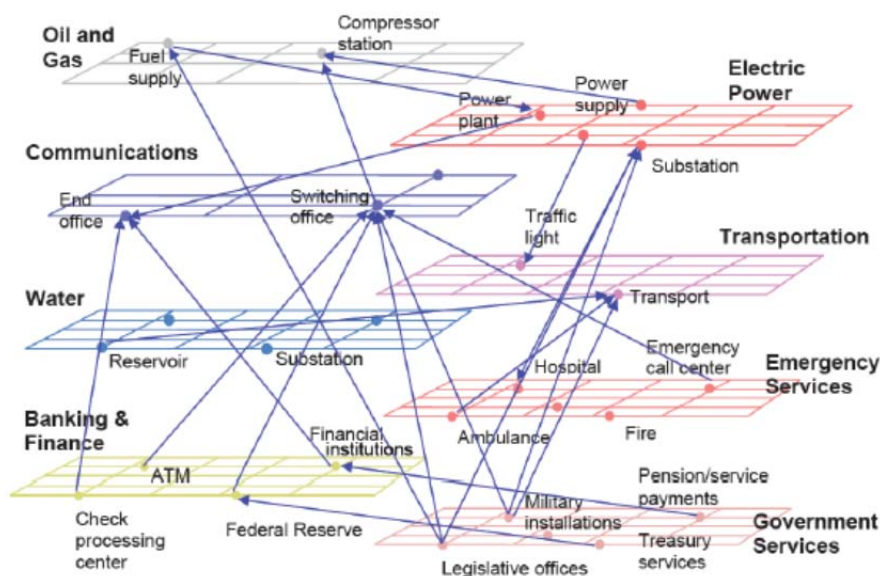
Figure 20 A Dynamic Interdependency Analysis of Critical Infrastructure Conceptual Diagram: OECD (2012) Identifying Bottlenecks and Prioritizing their Resolution
